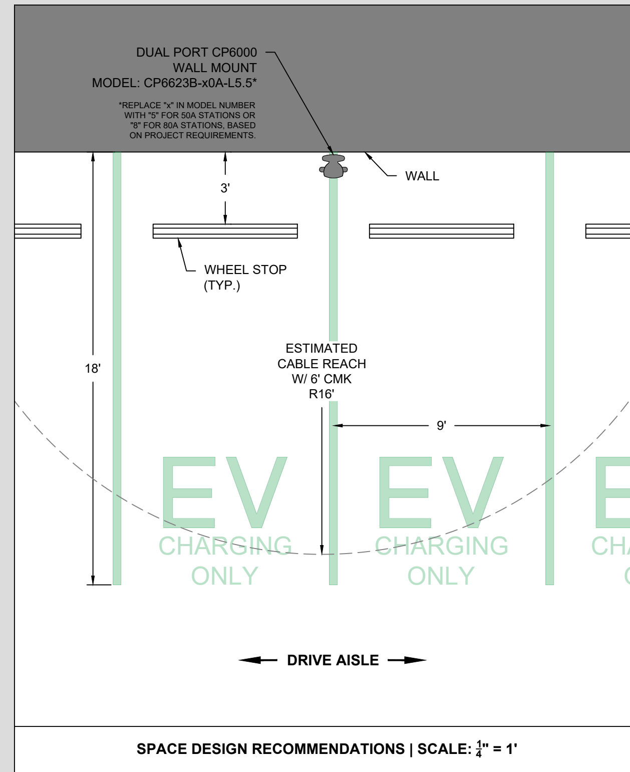
4 - WALL MOUNTED STATIONS
