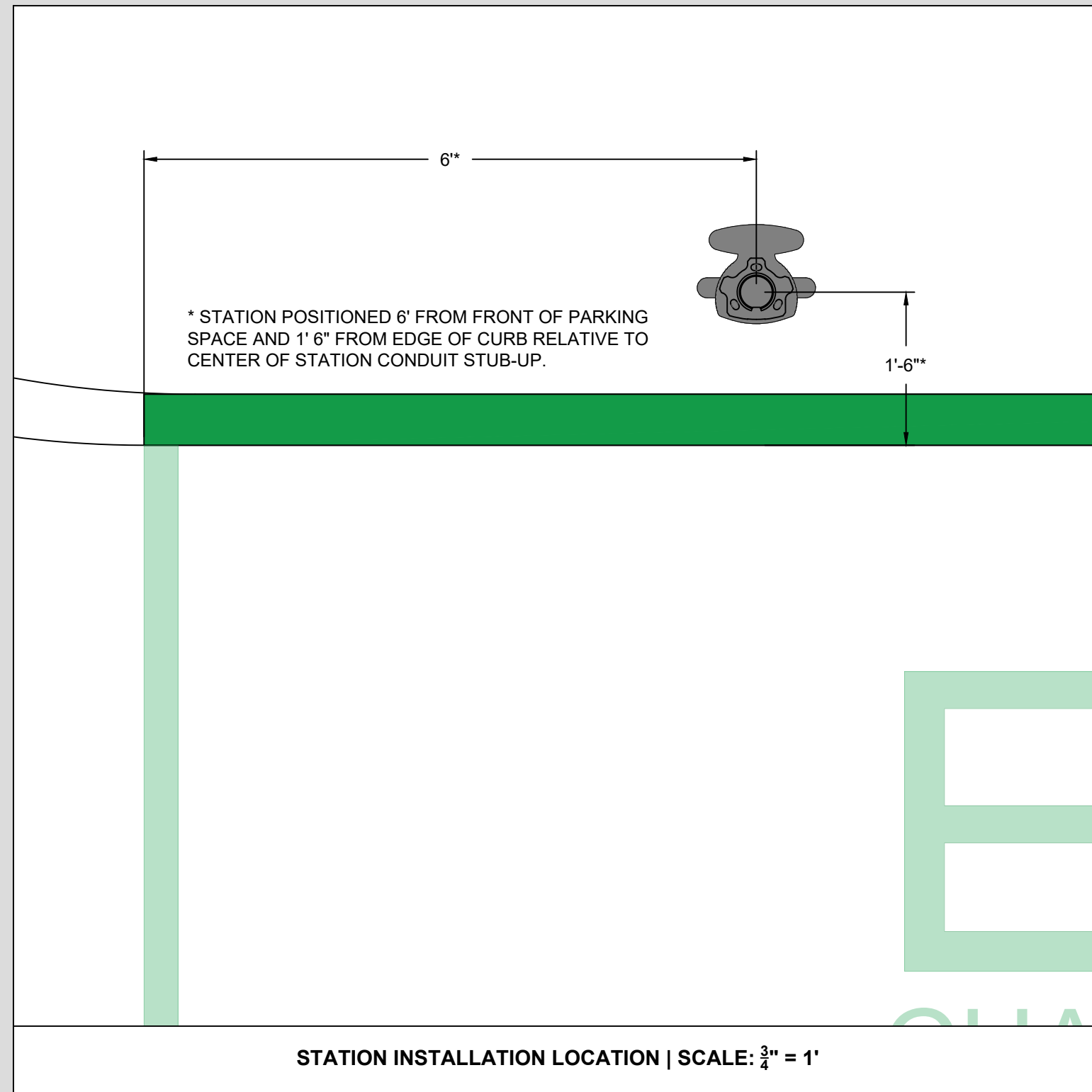
1 - SINGLE PARALLEL PARKING SPACE
