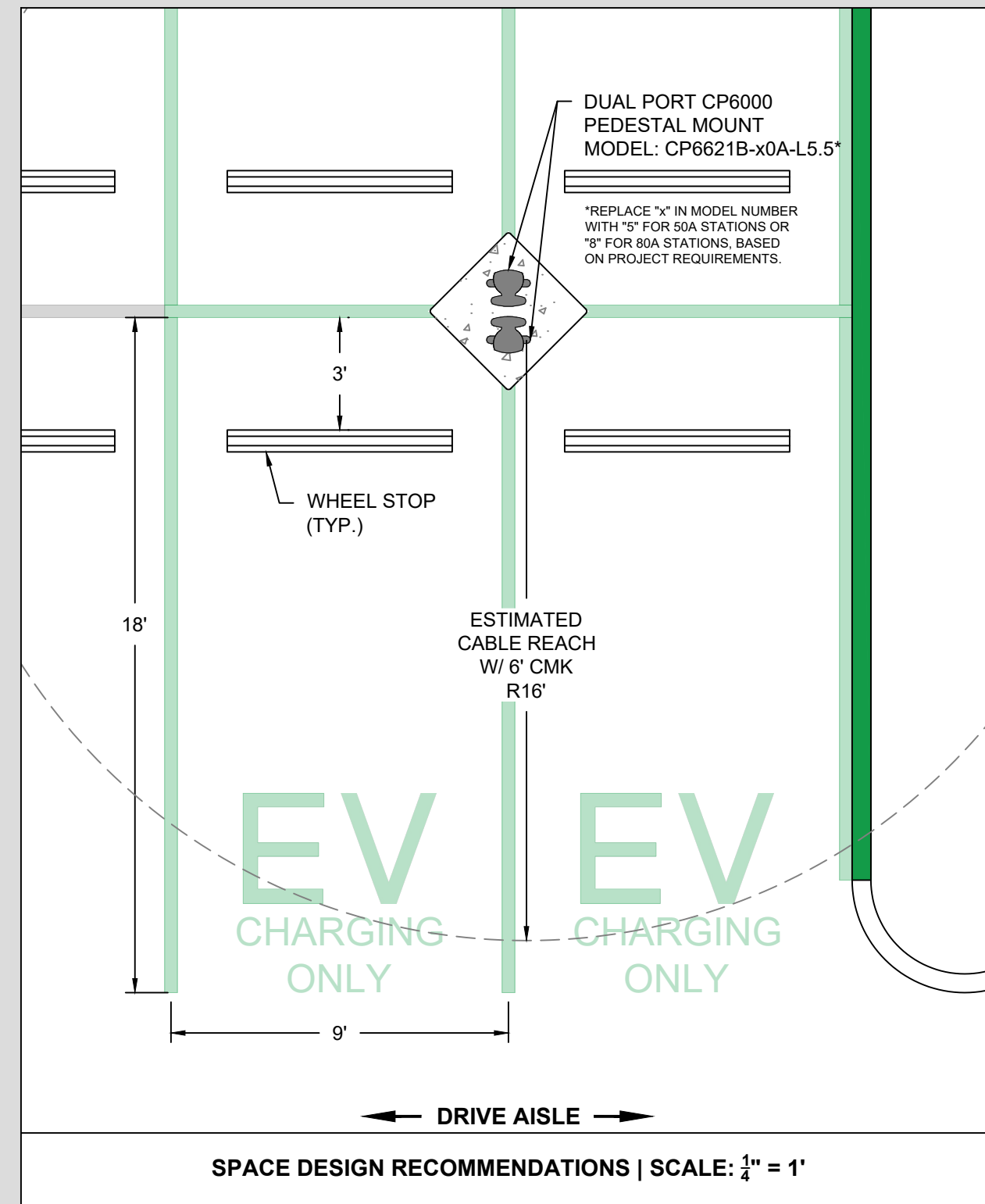
2 - STATIONS BETWEEN FOUR SPACES
