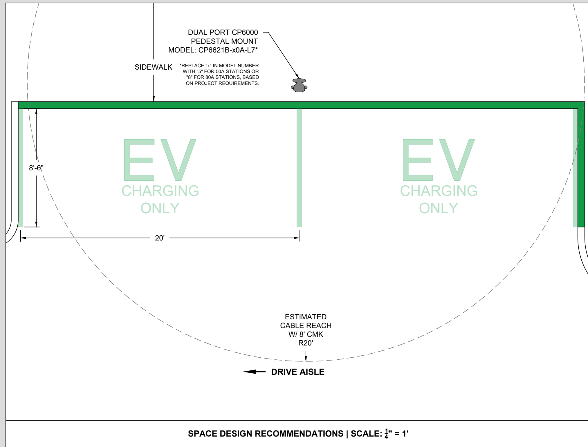
2 - MULTIPLE PARALLEL PARKING SPACES
