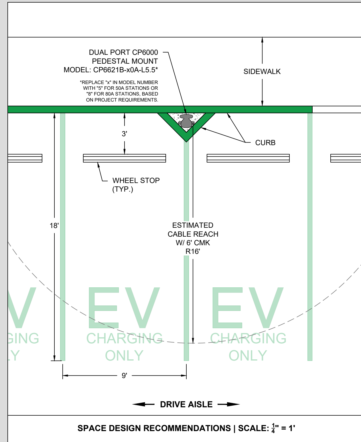
1 - STATION INSTALLED IN FRONT OF CURB
