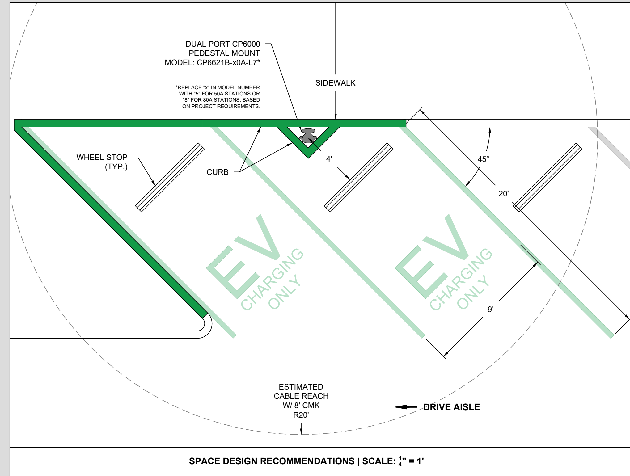
3 - DIAGONAL PARKING SPACES (45°)
