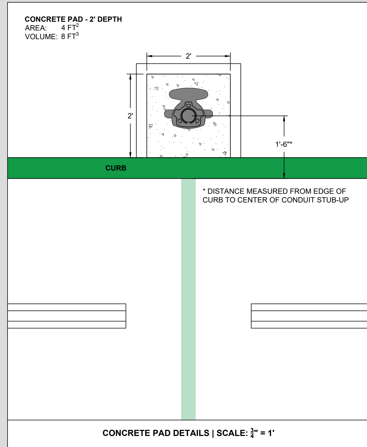
3 - STATION INSTALLED BEHIND CURB
