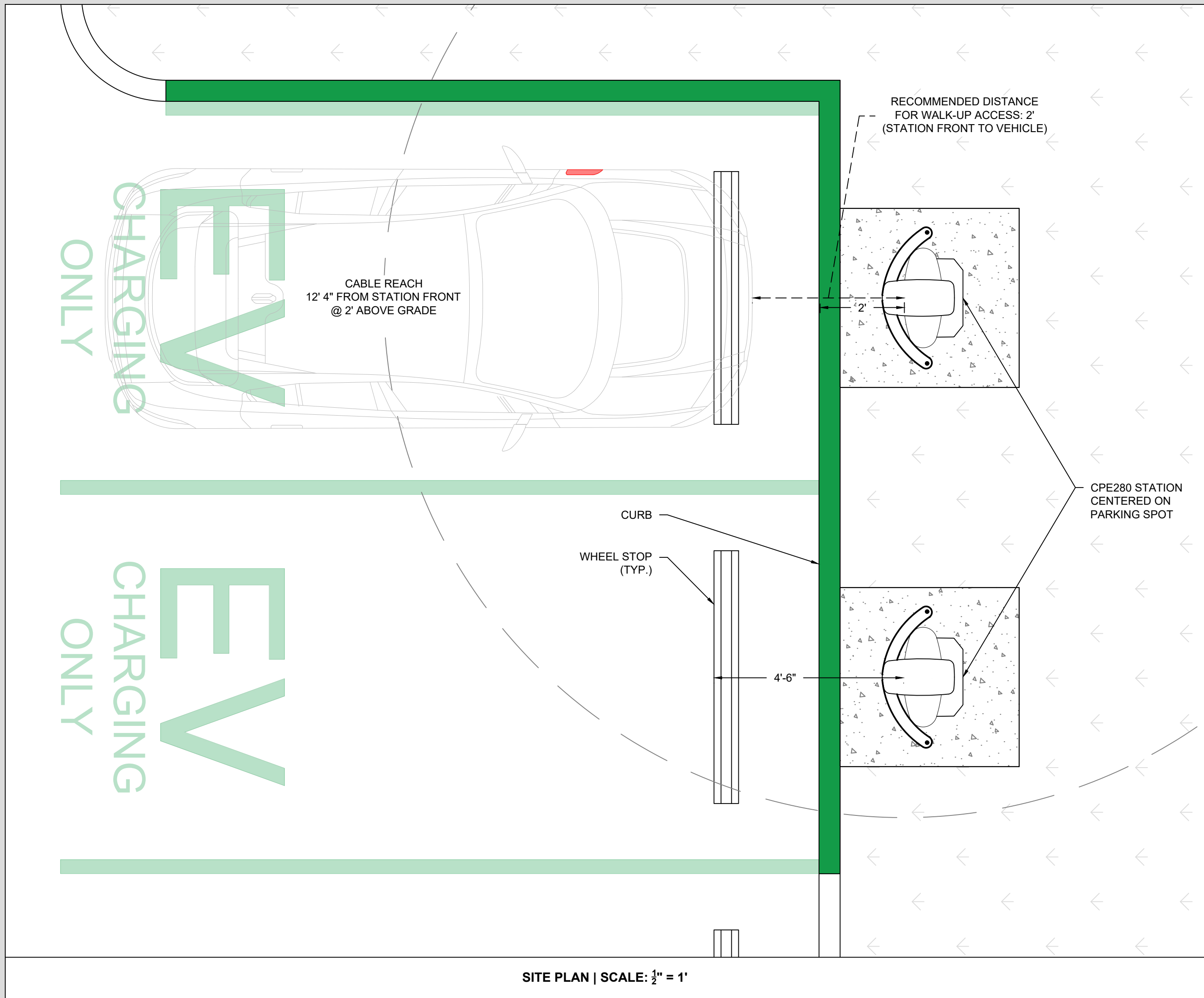
1 - PULL-IN PARKING SPACES
