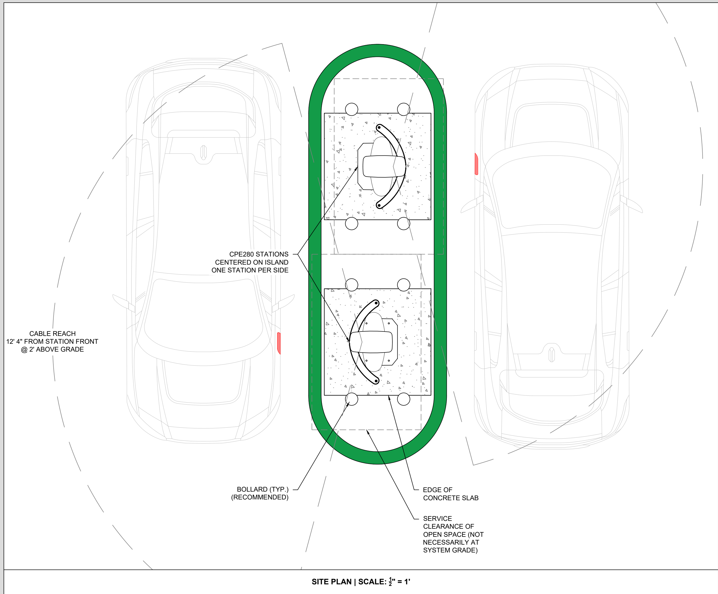
2 - CHARGING ISLANDS
