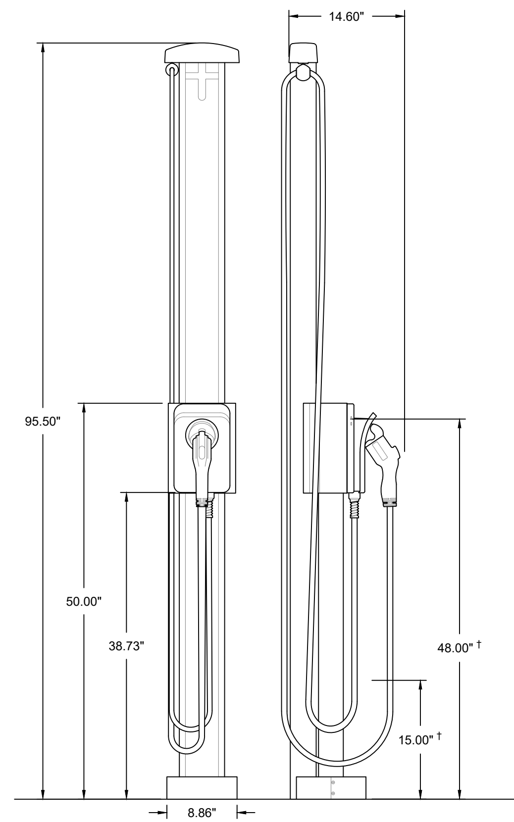
6A SINGLE PORT - PEDESTAL MOUNT WITH CABLE MANAGEMENT CONCRETE MOUNTING SECTION (23' CABLE) | SCALE: 1" = 1'0"
