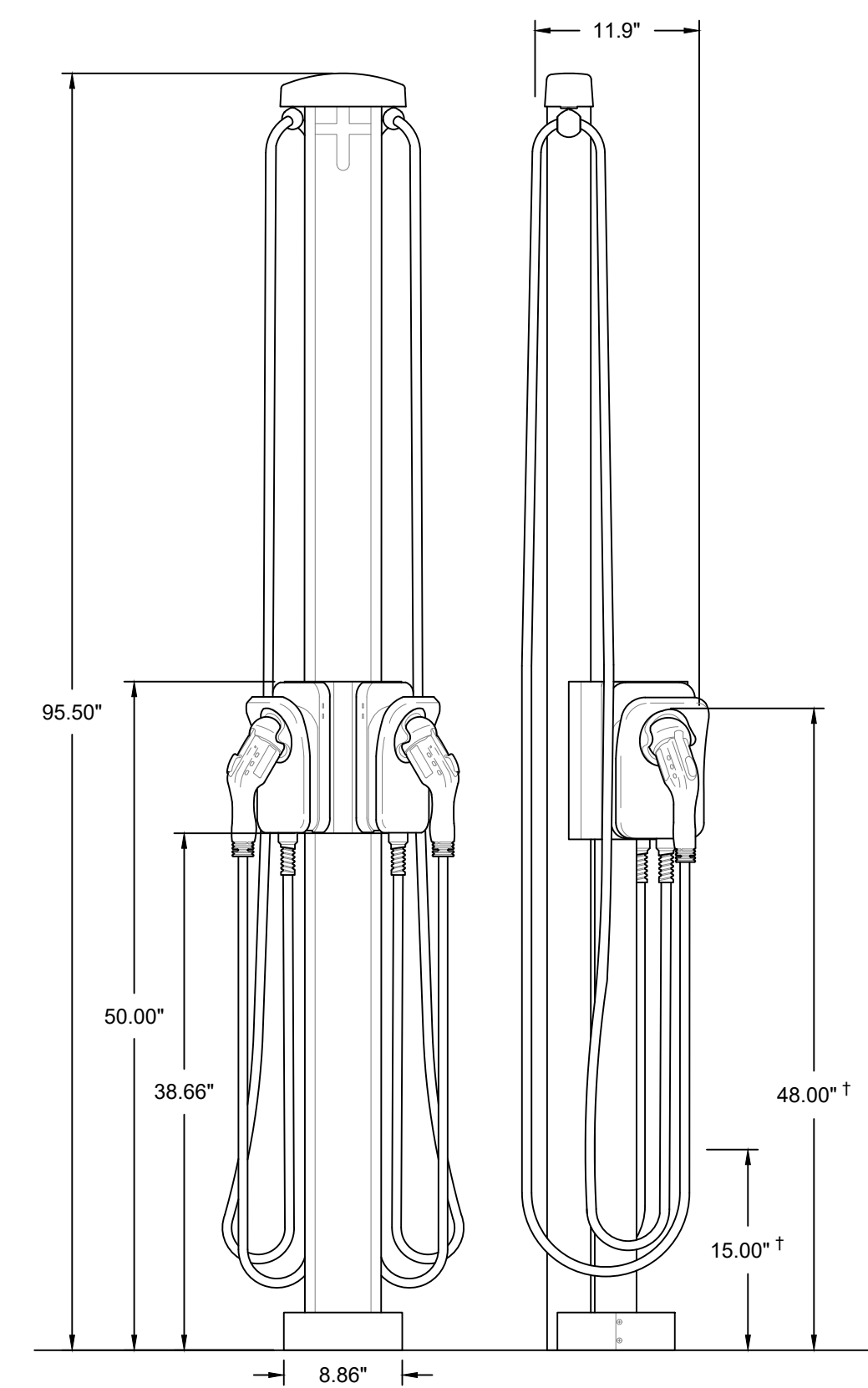
7A DUAL PORT - PEDESTAL MOUNT WITH CABLE MANAGEMENT CONCRETE MOUNTING SECTION (23' CABLES) | SCALE: 1" = 1'0"
