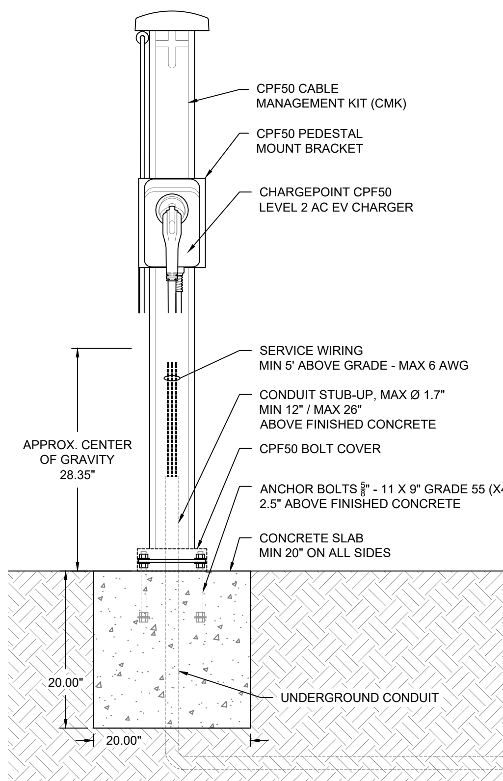
4A SINGLE PORT - PEDESTAL MOUNT WITH CABLE MANAGEMENT CONCRETE MOUNTING SECTION (18' CABLE) | SCALE: 1" = 1'0"
