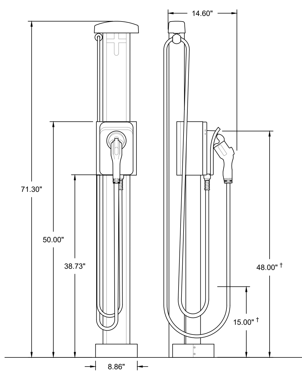
4B SINGLE PORT - PEDESTAL MOUNT WITH CABLE MANAGEMENT ELEVATIONS (18' CABLE) | SCALE: 1" = 1'0"
