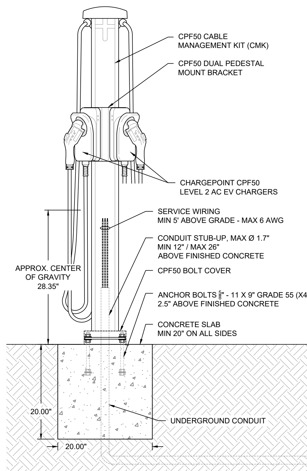
5A DUAL PORT - PEDESTAL MOUNT WITH CABLE MANAGEMENT CONCRETE MOUNTING SECTION (18' CABLES) | SCALE: 1" = 1'0"
