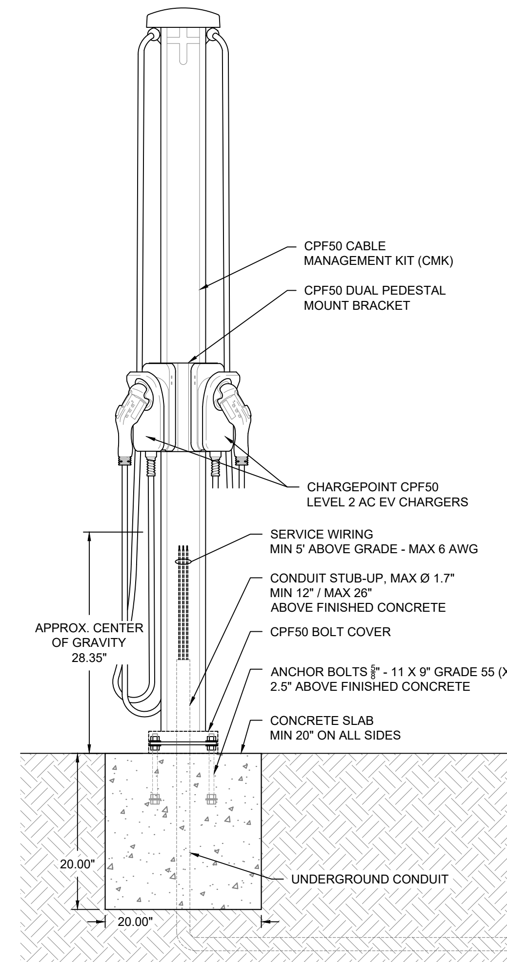
7A DUAL PORT - PEDESTAL MOUNT WITH CABLE MANAGEMENT CONCRETE MOUNTING SECTION (23' CABLES) | SCALE: 1" = 1'0"
