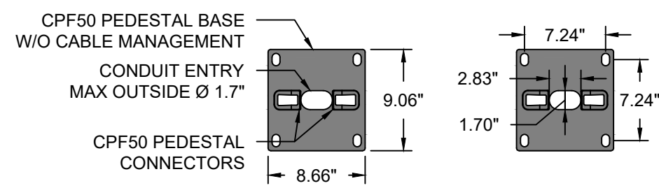
1 PEDESTAL WITHOUT CABLE MANAGEMENT - MOUNTING HOLE PATTERN SCALE: 1" = 1'0"
