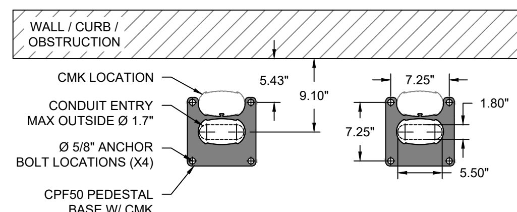
2 PEDESTAL WITH CABLE MANAGEMENT - MOUNTING HOLE PATTERN SCALE: 1" = 1'0"
