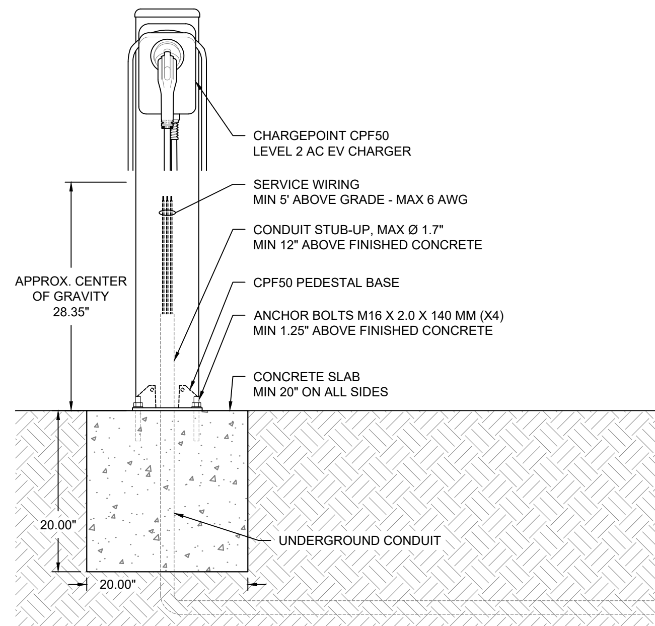
3A SINGLE AND DUAL PORT - PEDESTAL MOUNT WITHOUT CABLE MANAGEMENT CONCRETE MOUNTING SECTION | SCALE: 1" = 1'0"
