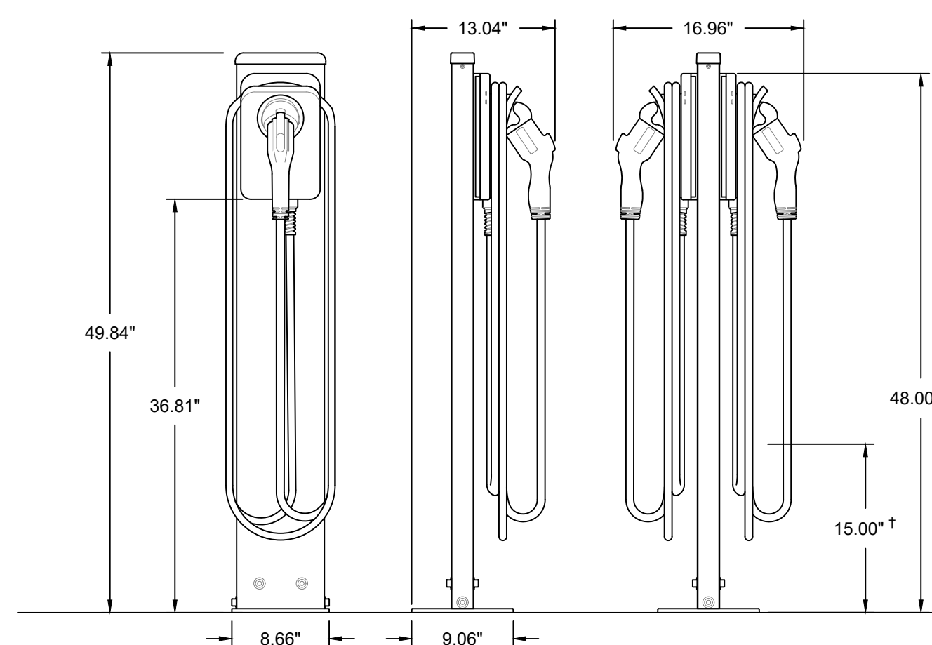
3B SINGLE AND DUAL PORT - PEDESTAL MOUNT WITHOUT CABLE MANAGEMENT ELEVATIONS | SCALE: 1" = 1'0"
