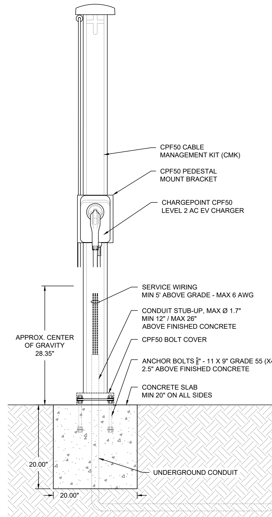
6A SINGLE PORT - PEDESTAL MOUNT WITH CABLE MANAGEMENT CONCRETE MOUNTING SECTION (23' CABLE) | SCALE: 1" = 1'0"
