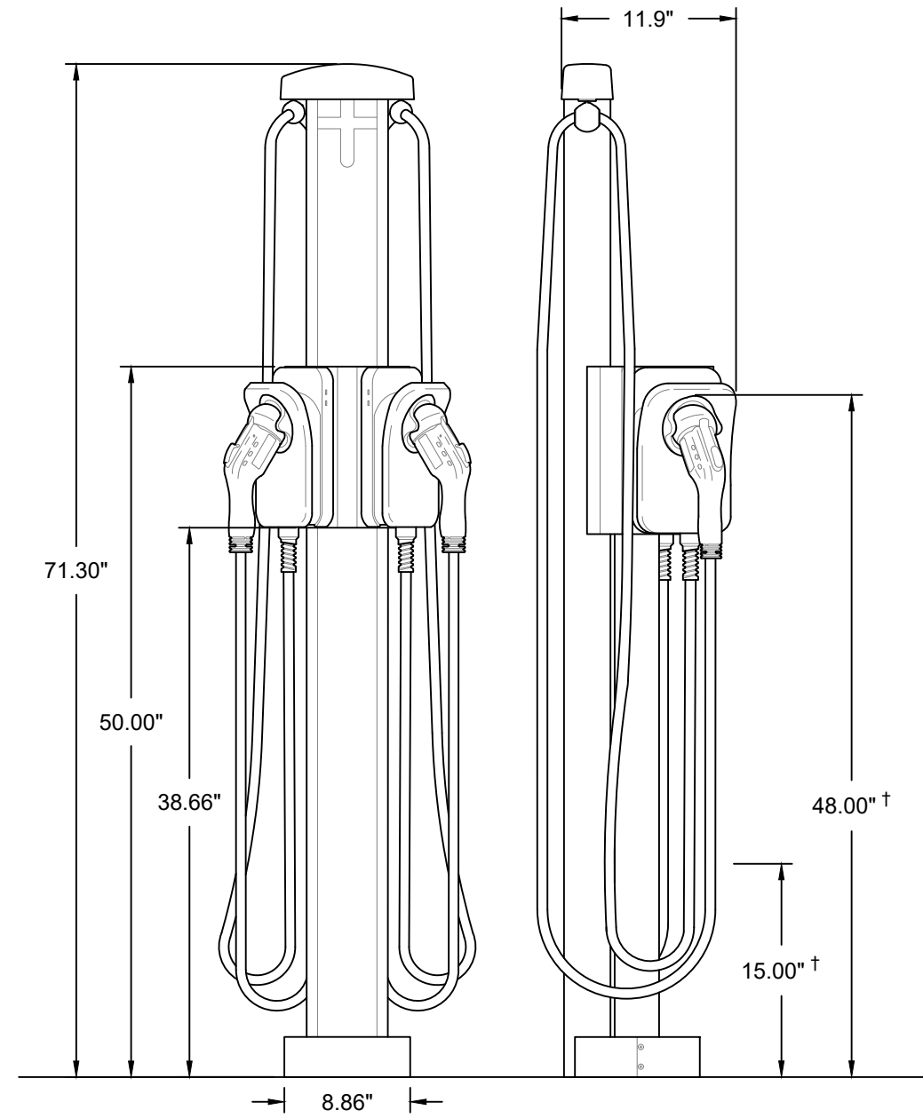
5B DUAL PORT - PEDESTAL MOUNT WITH CABLE MANAGEMENT ELEVATIONS (18' CABLES) | SCALE: 1" = 1'0"
