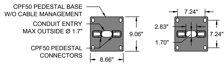
10 PEDESTAL MOUNT WITHOUT CABLE MANAGEMENT MOUNTING HOLE PATTERN | SCALE: 1" = 1'0"
