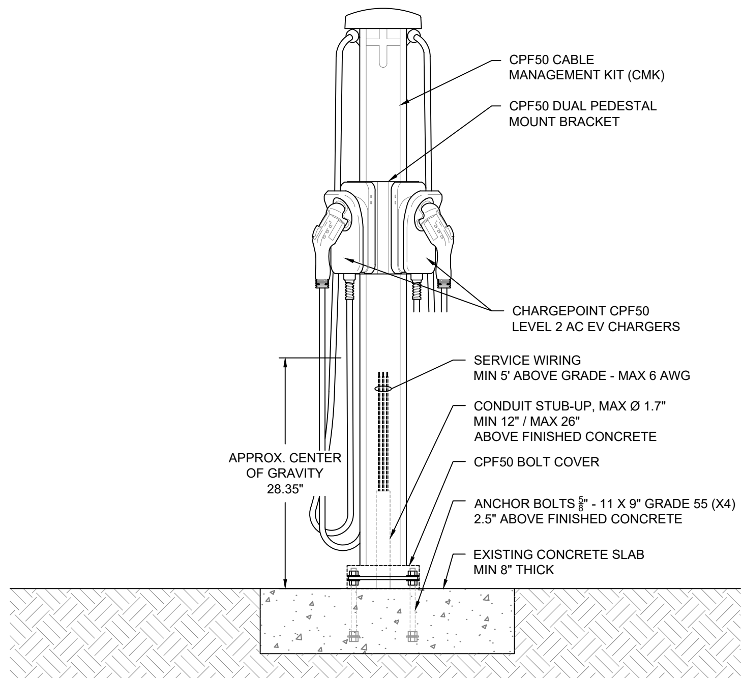
29 PEDESTAL MOUNT WITH CABLE MANAGEMENT CONCRETE MOUNTING SECTION - EXISTING CONCRETE | SCALE: 1" = 1'0"
