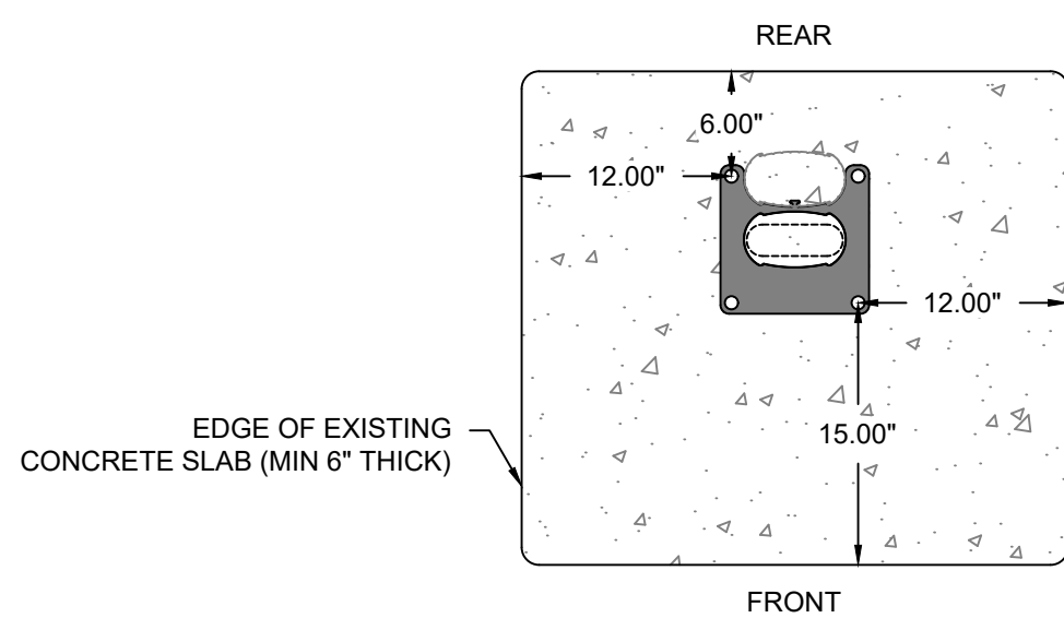
28 PEDESTAL MOUNT WITH CABLE MANAGEMENT MOUNTING CLEARANCES - EXISTING CONCRETE | SCALE: 1" = 1'0"
