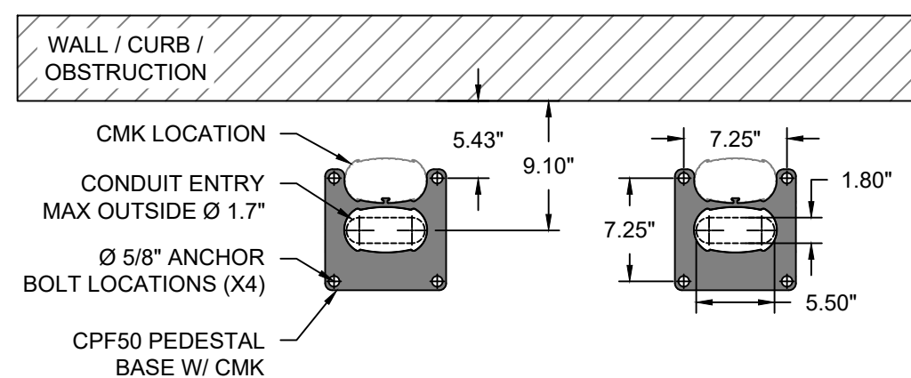
20 PEDESTAL MOUNT WITH CABLE MANAGEMENT MOUNTING HOLE PATTERN | SCALE: 1" = 1'0"
