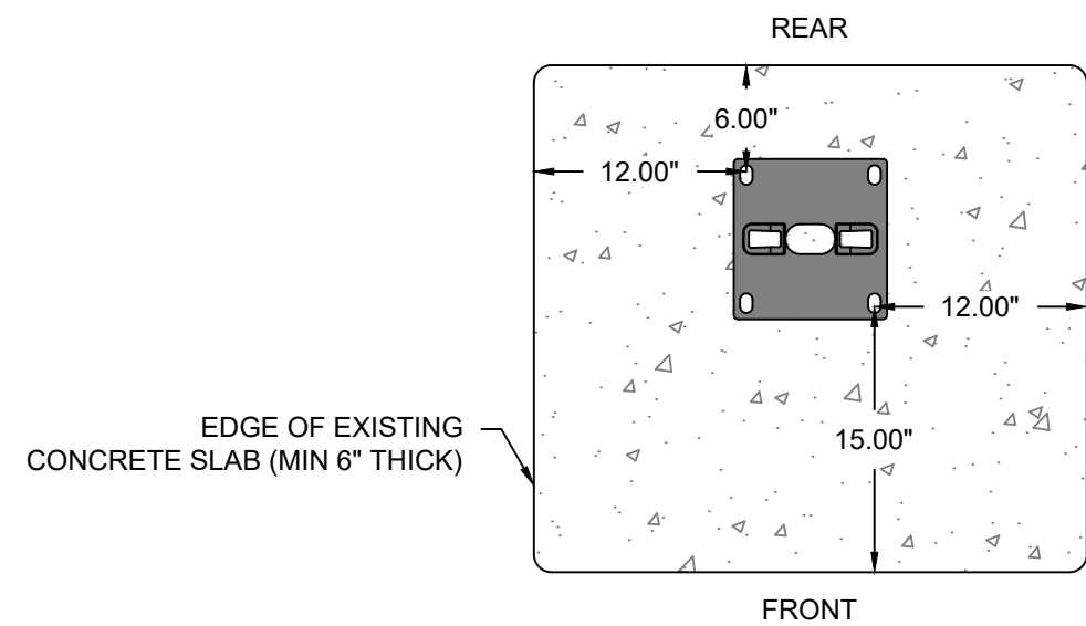
18 PEDESTAL MOUNT WITHOUT CABLE MANAGEMENT MOUNTING CLEARANCES - EXISTING CONCRETE | SCALE: 1" = 1'0"
