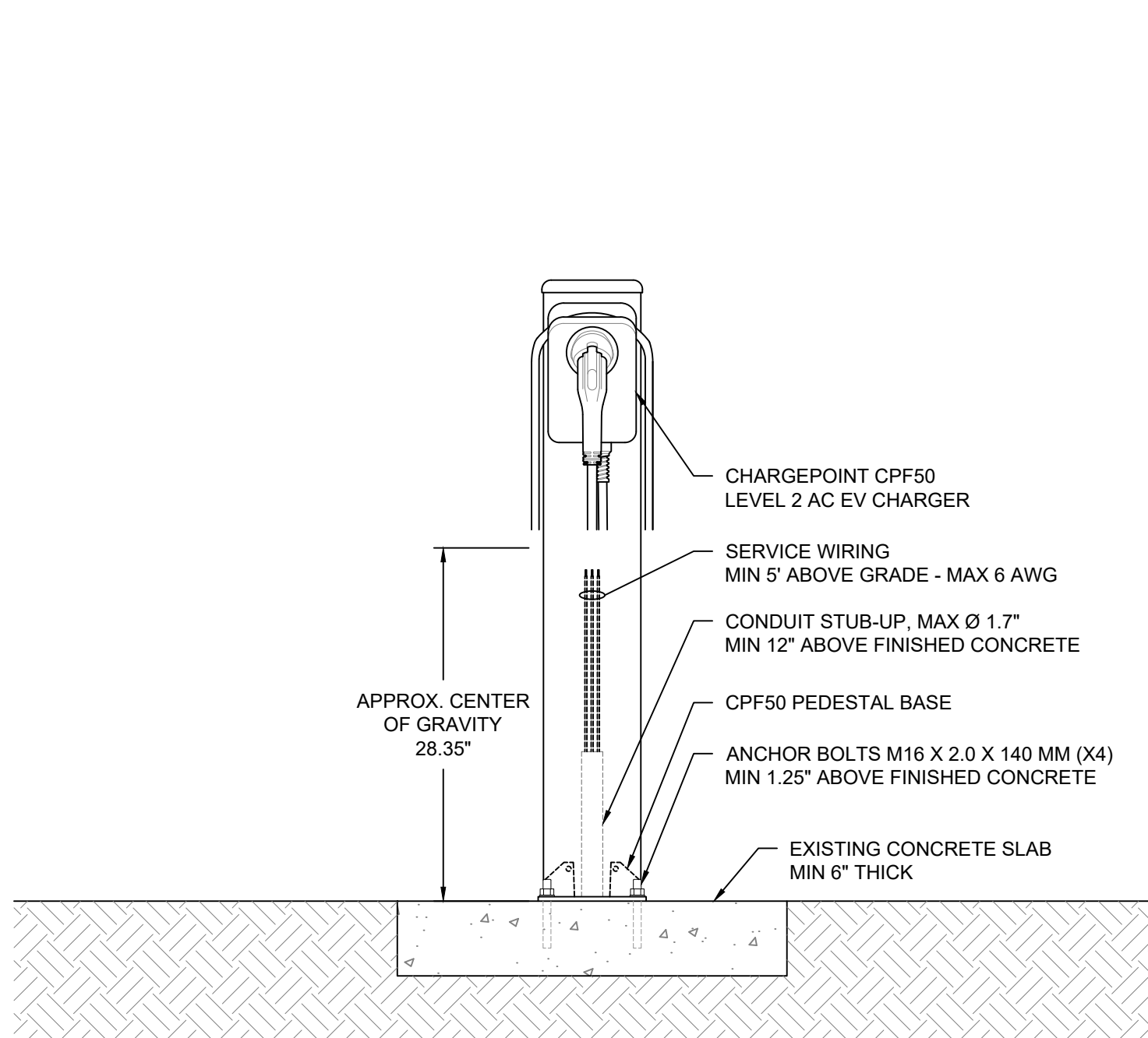
19 PEDESTAL MOUNT WITHOUT CABLE MANAGEMENT CONCRETE MOUNTING SECTION - EXISTING CONCRETE | SCALE: 1" = 1'0"
